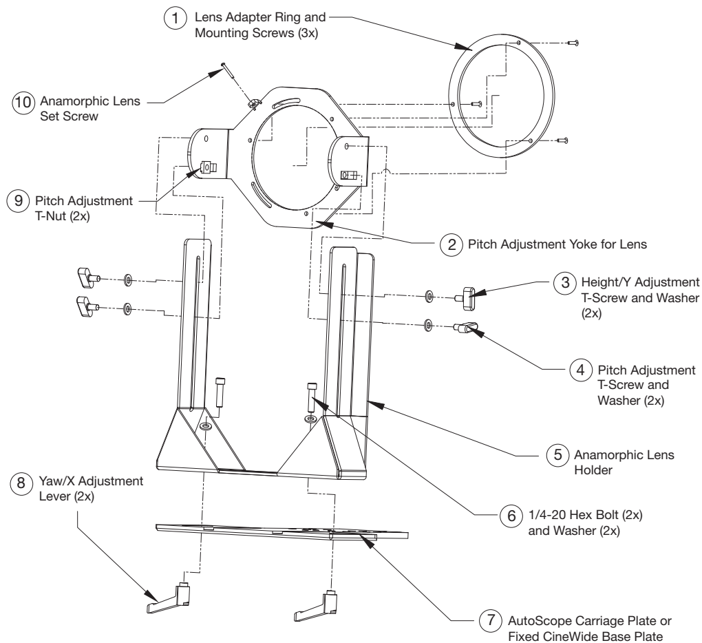
Figure 3-18. VX-22i Anamorphic Lens Mounting Assembly - Exploded View
