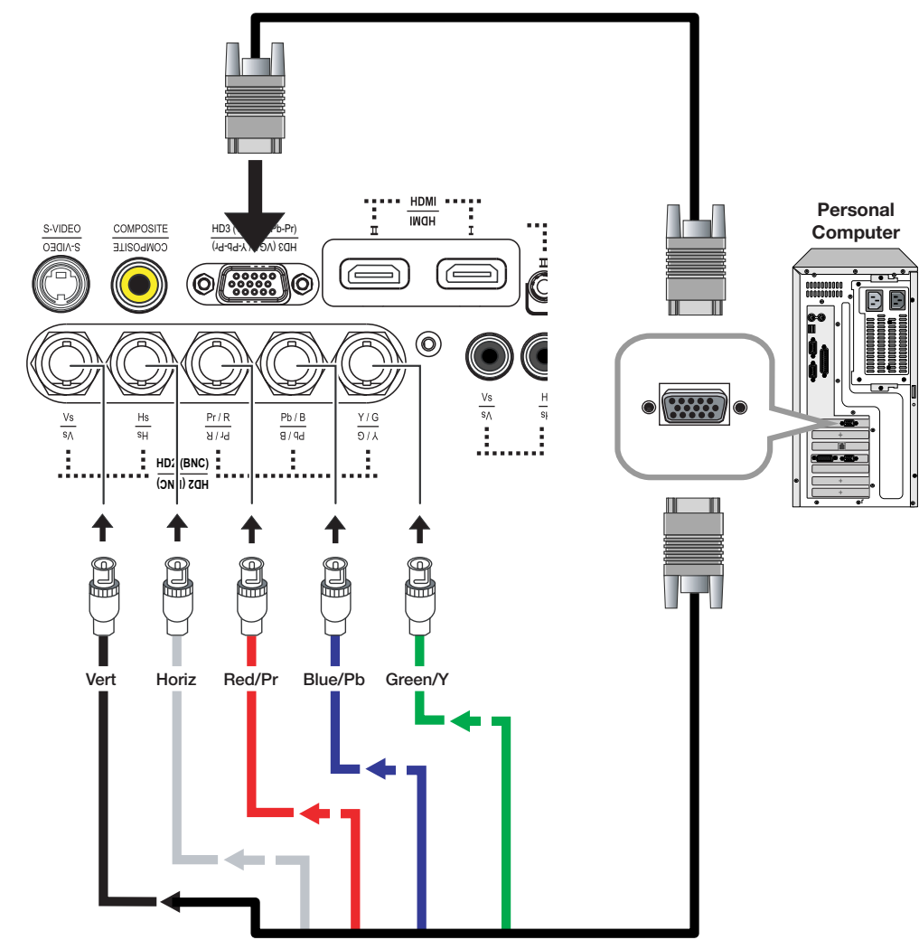
Figure 3-13. Analog RGB Connections
